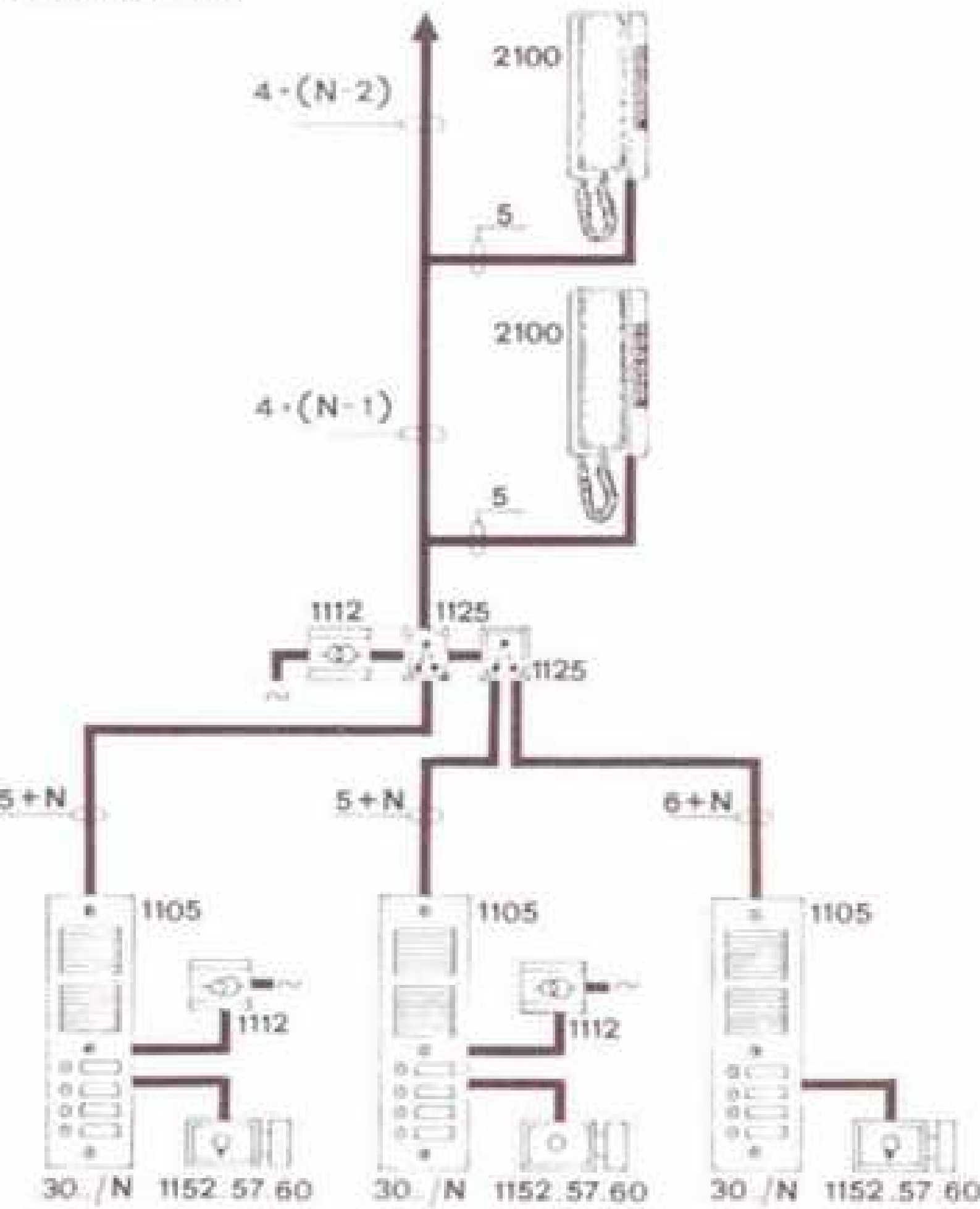
Door entry system with 3 entrances
