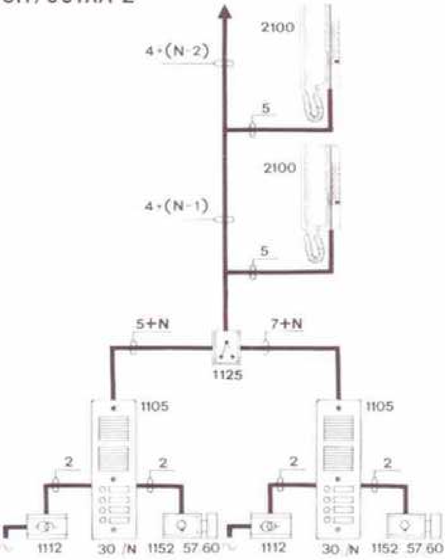
Door entry system with 2 entrances
